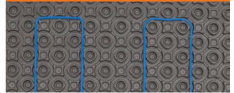
3- and 4-shape spacing = 10.6 W/ft 2
