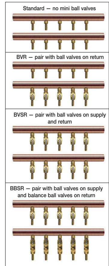
Ball valves with mini balancing valves are useful for exact flow balancing. Balancing is accomplished by rotating the threaded spindle below the brass safety cap. Each turn represents approximately 10% of full flow.
