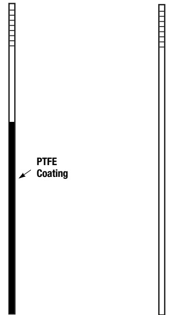
P-SS Probes
